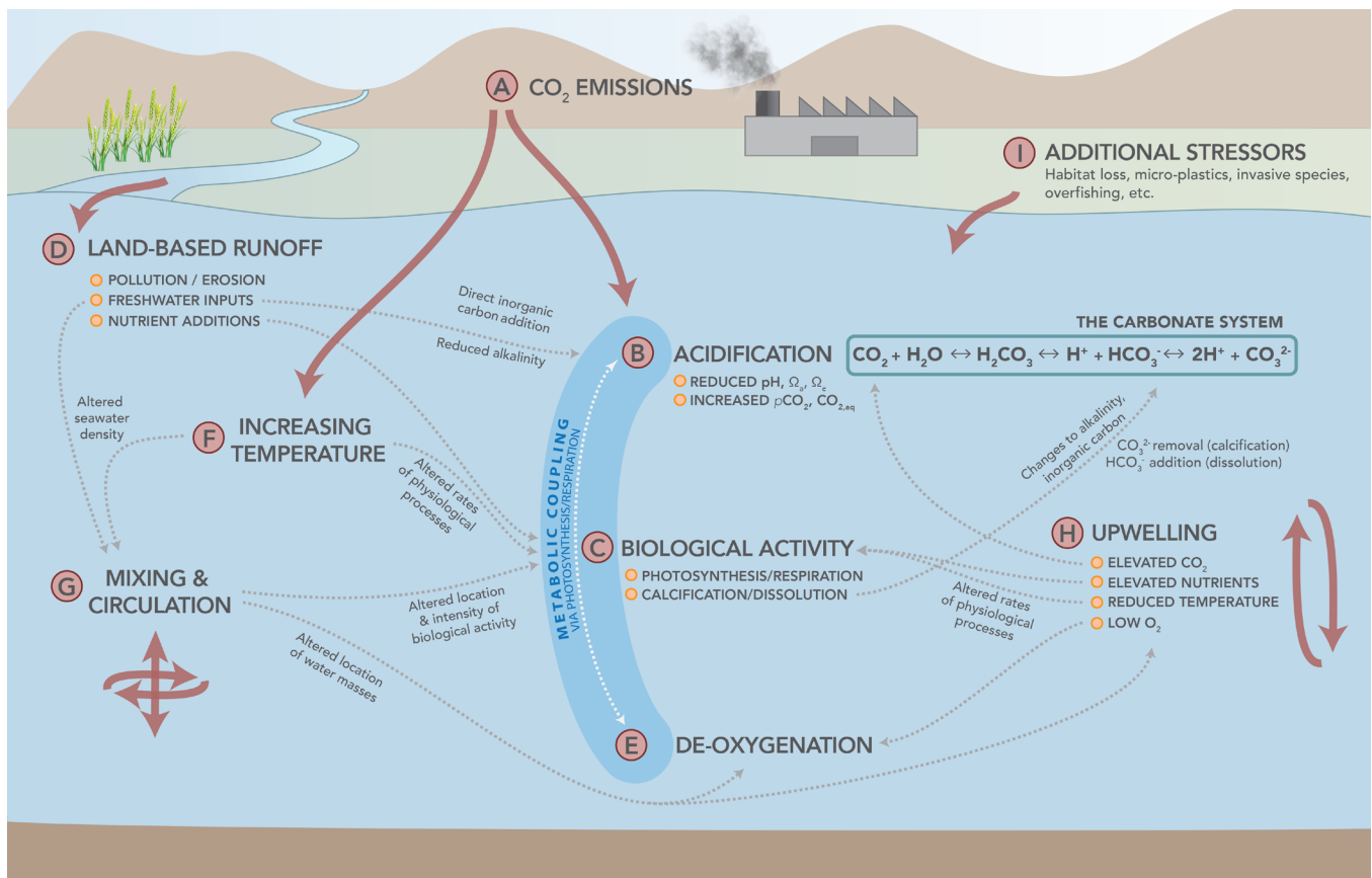
Figure 1. Overview of the major driving processes (and associated linkages among them) in coastal oceans. (A) Atmospheric CO 2 -driven (B) acidification occurs against a backdrop of additional drivers of change in ocean conditions, including (D) land-based runoff, (E) deoxygenation, (F) warming, (G) mixing and circulation, (H) upwelling, and (I) other additional stressors. Processes can be accentuated in bodies of water with low circulation and mixing, for example tidal flushed bays and estuaries, as well as tidepools.
